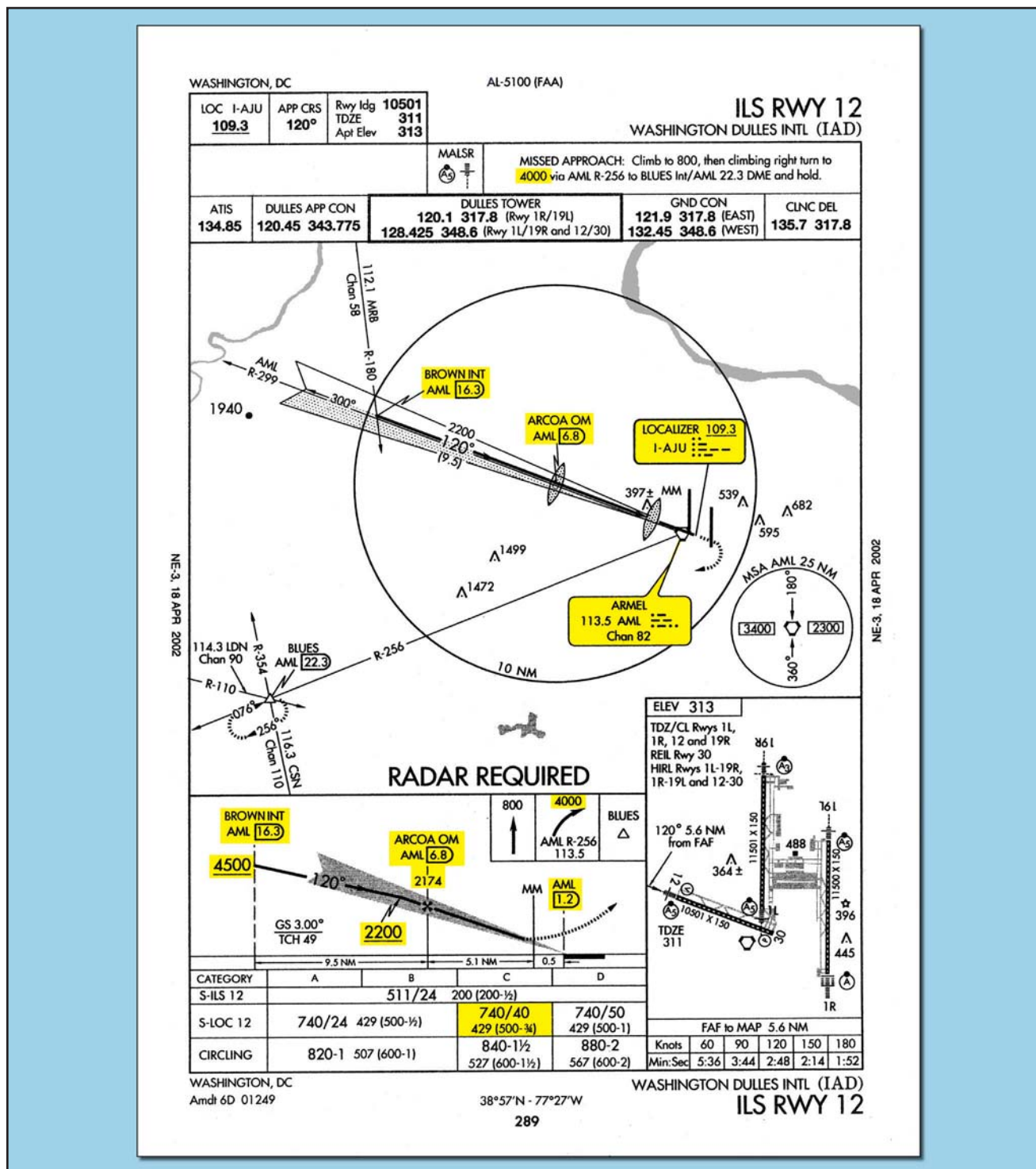
Figure 5-18. Example Approaches Using Autopilot.
