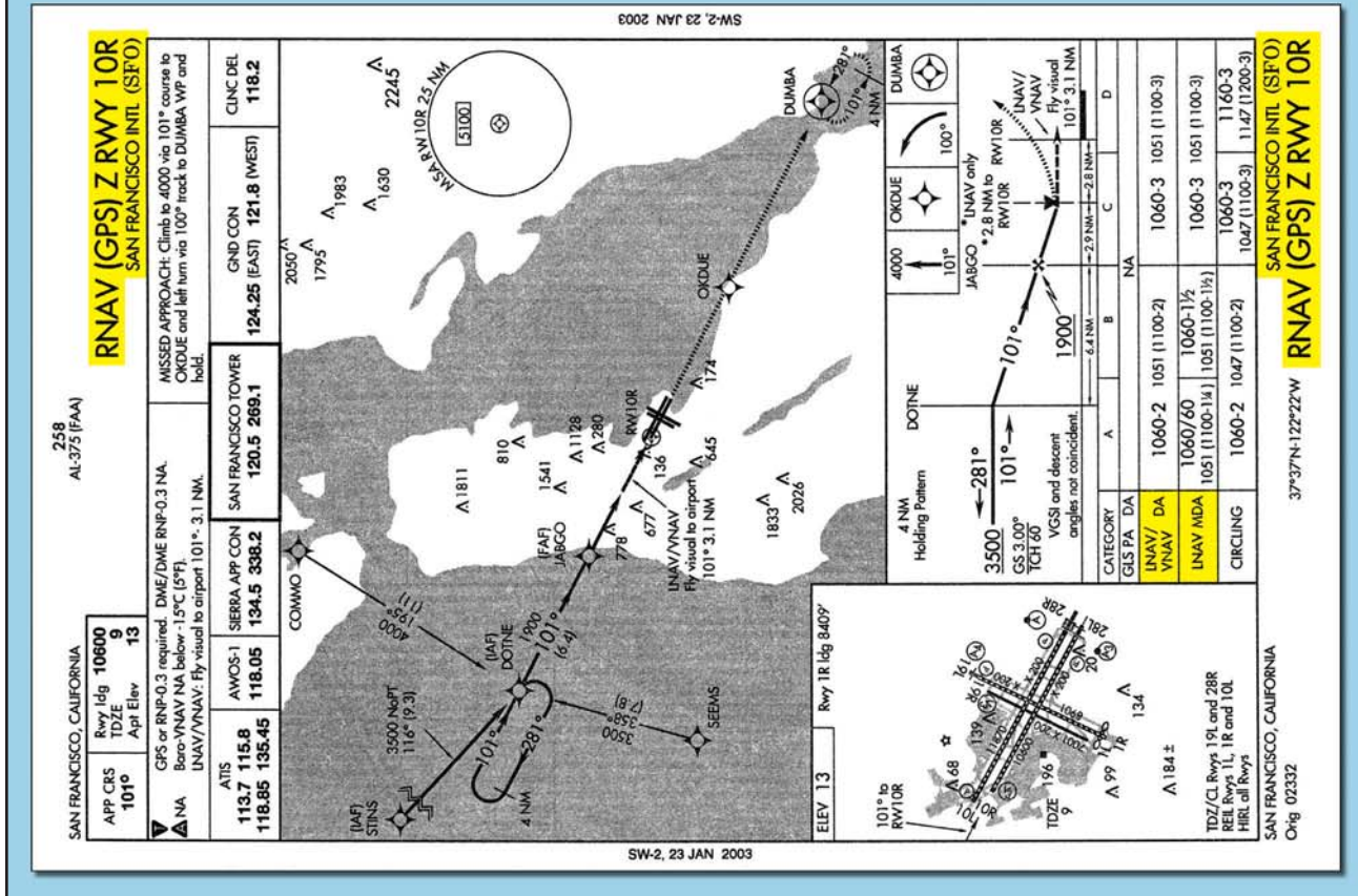
Figure 5-5. Multiple Approaches.
