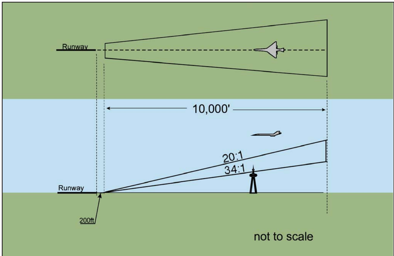
Figure 5-19. Determination of Visibility Minimums.
