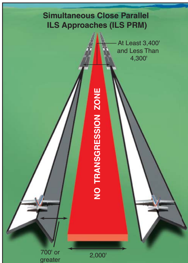
Figure 5-42. Simultaneous Close Parallel ILS Approach (ILS PRM) Criteria.
