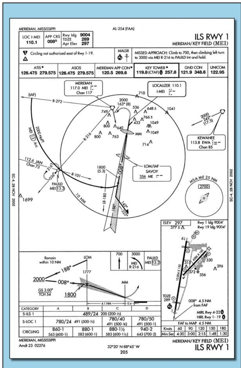
Figure 5-3. Pilot Briefing Information NACO Chart Format.
